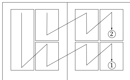
Taco: columnset blocks taking input from streams
